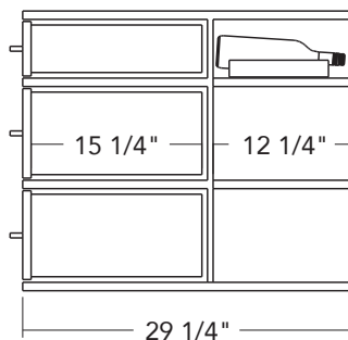
Cross Section
