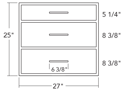
Drawer Side
